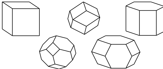
Figure 10: Parallelohedra in \mathbb{R}^3 .
